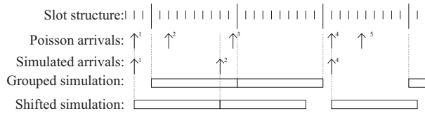
Fig. 2. Illustration of the arrival process of a single user, as used by the simulation. Poisson arrivals 3 and 5 are not considered in the simulation, since they are both the second arrival within the same group. Although arrival 2 occurs shortly after the first one, it is used, but assumed to arrive exactly N slots after the first one. Thus, both simulations consider the same arrivals as used in the theoretical analysis.
